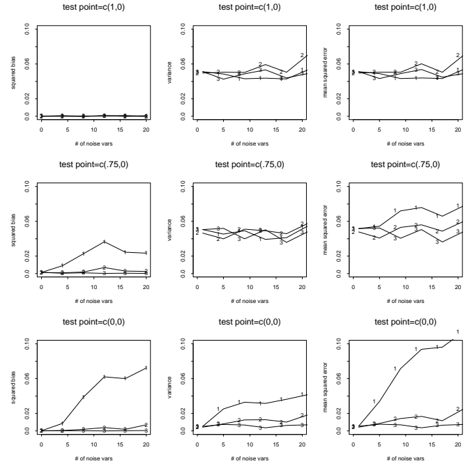
Fig. 10. Bias, variance and mean squared error of 5-NN (1), DANN (2) and 5-NN restricted to the first predictor (3). There are two classes with centers (0,0) and (2,0) . In the top, middle and bottom rows the prediction is done at (1,0) , (.75,0) and (0,0) respectively. The simulation standard errors of the bias and variance estimates are roughly .015 and .003 respectively.
