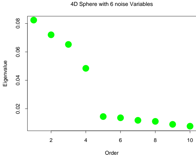
Fig. 4. The eigenvalues of the average between matrix for the 4D sphere + 6 noise variable problem. Using these first four dimensions followed by our DANN nearest neighbor routine, we get better performance than 5NN in the real 4D subspace.
